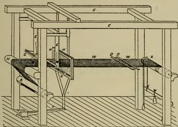
DIAGRAM OF A HAND LOOM
